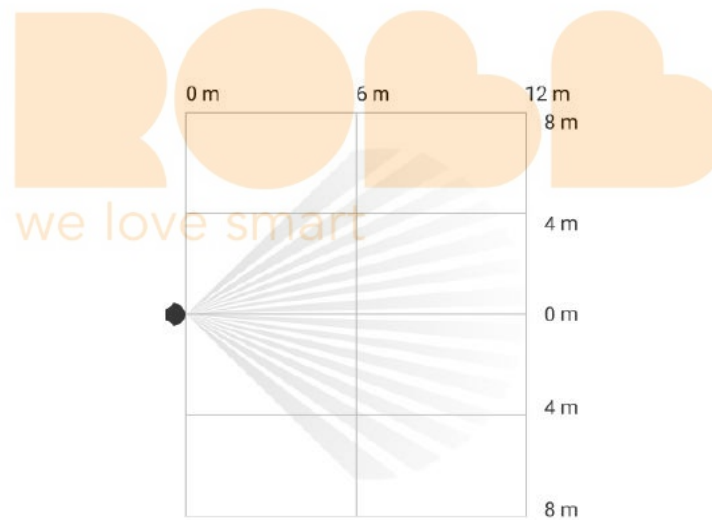
Horizontal viewing angle of the detector
